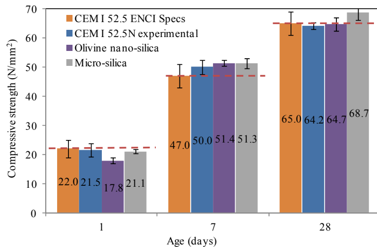
Figure 6. Compressive strength development of the tested mortars.
