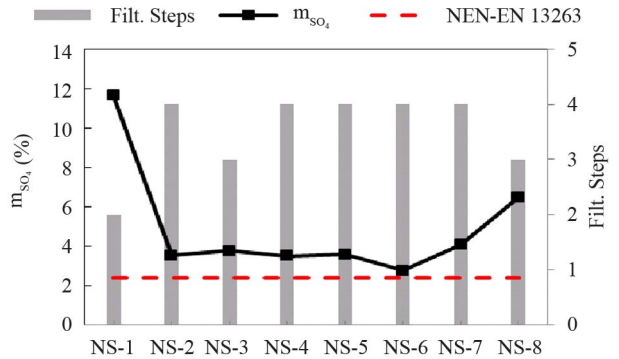
Figure 4. Sulfate content in olivine nano-silicas, sulfate limited by the norm and filtration steps.
